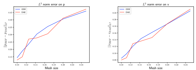
(a) L^2 pressure error.
