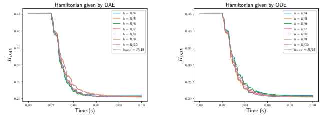
(a) DAE system (21).
