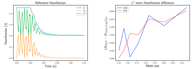
(a) Reference Hamiltonian.
